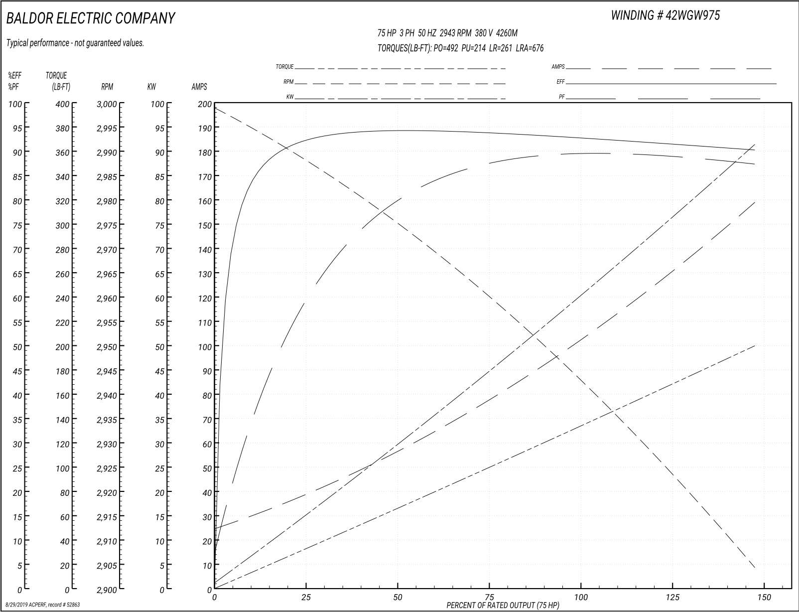
Performance Graph at 380V, 50Hz, 75.0HP Typical performance - Not guaranteed values
